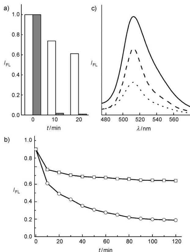
Figure 3. a) Decay in the relative fluorescence intensity ( I_{FL} ) for free EGFP (filled bar) and silica-NP-encapsulated EGFP (empty bar) in 6 M GdHCl. b) The relative I_{FL} decay for free EGFP (○) and silica-NP-encapsulated EGFP (□) on treatment with protease K. c) The fluorescence spectra of EGFP-Ca@SiO 2 at a EGFP-equivalent concentration of 0.25 mg mL -1 : newly prepared (solid line), suspension of dried EGFP-Ca@SiO 2 after storage for 70 days at room temperature (dotted line), the above suspension recorded after 96 h (dashed line).
